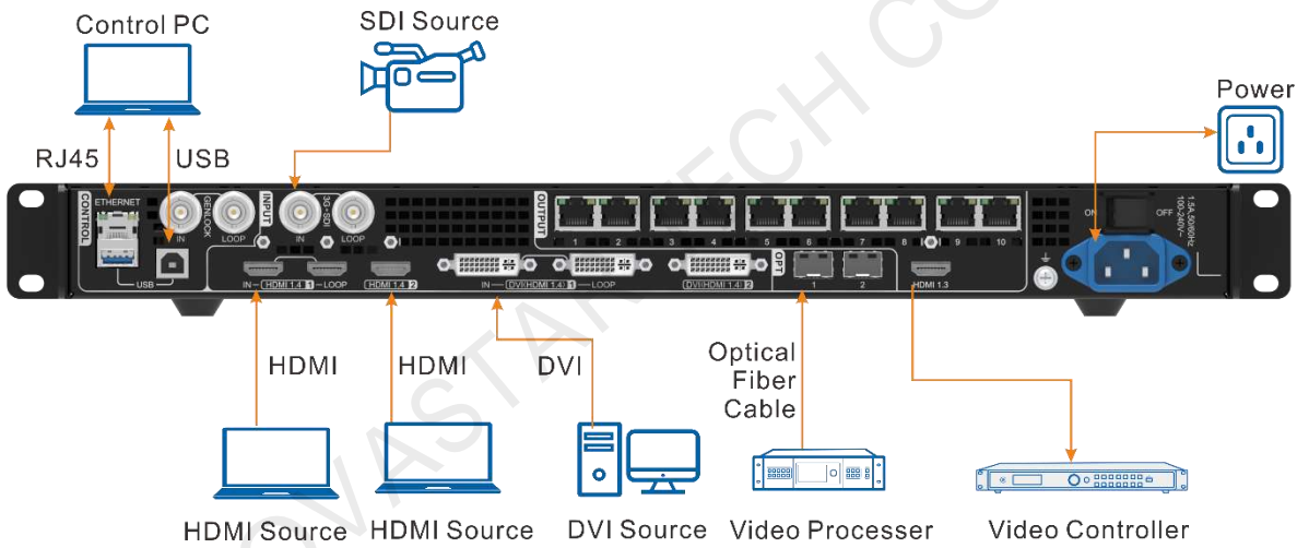
Figure 5-33 HDMI output
