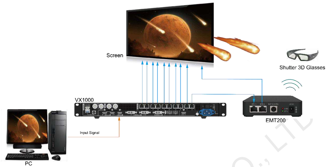
Figure 5-38 3D connections
