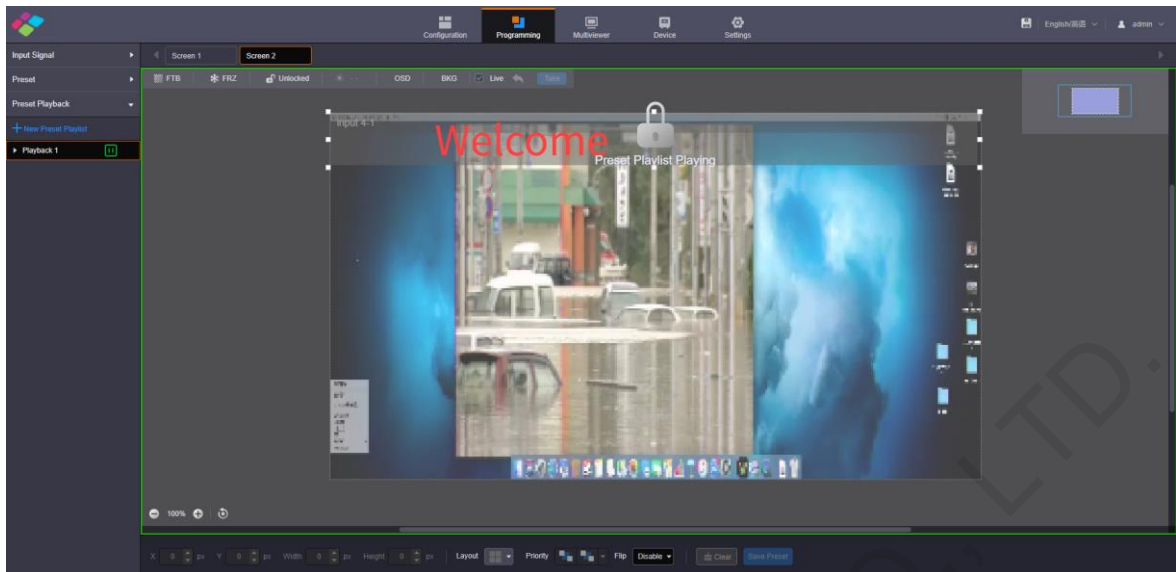
Figure 4-15 Playing presets
