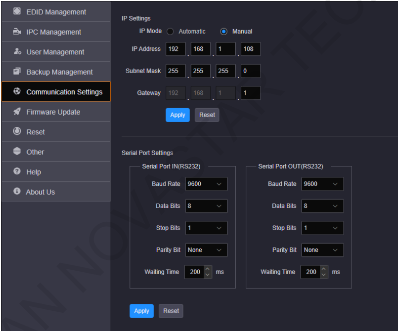
Figure 6-25 Communication settings
