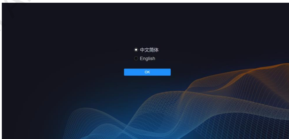
Figure 5-11 Web page
