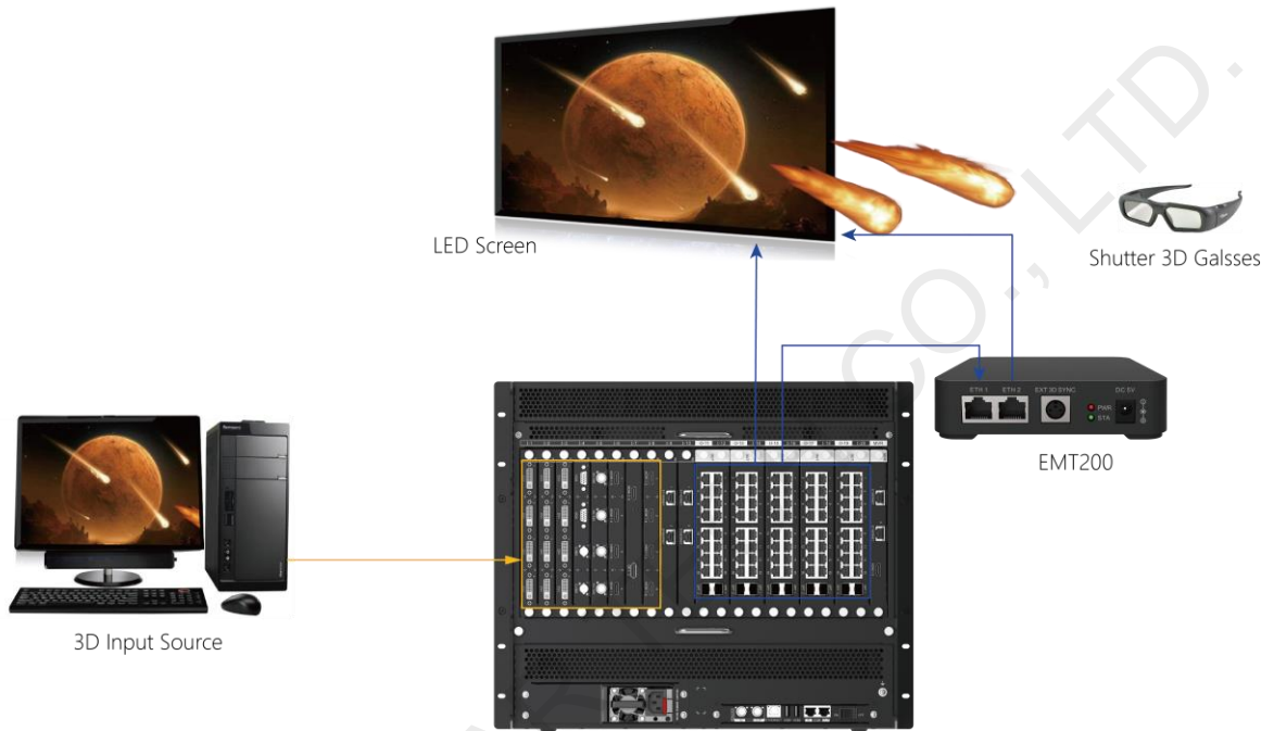
Figure 4-21 Hardware connections
