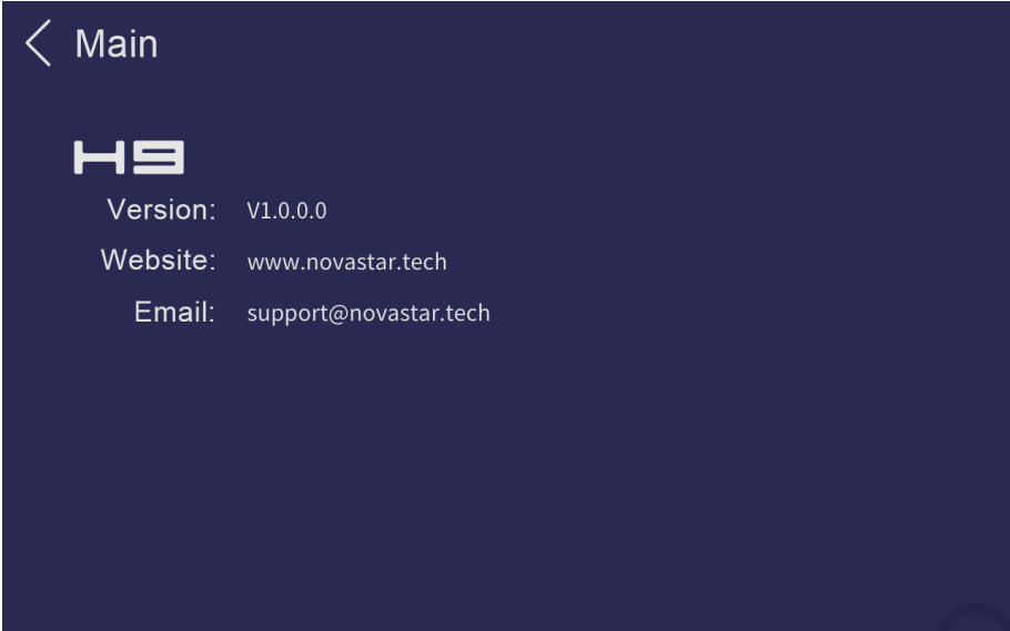
Figure 5-16 About us
