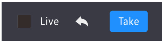
Figure 4-4 Pre-edit mode
