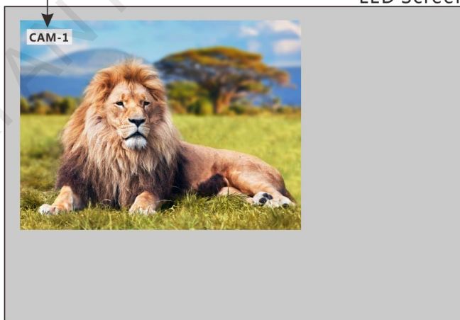
Figure 4-24 Channel logo
