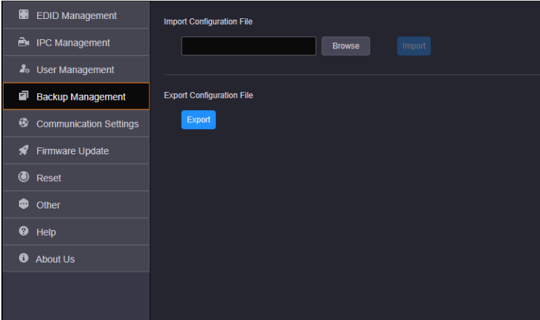
Figure 6-24 Backup management
