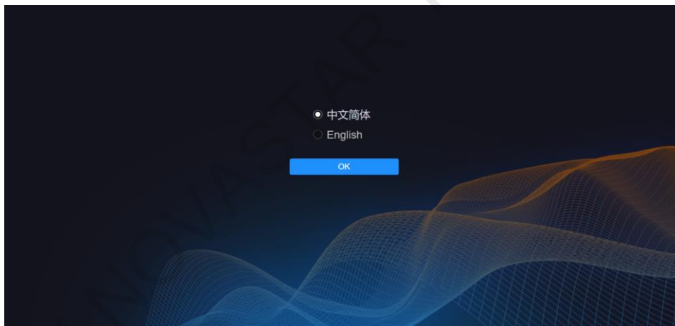
Figure 6-28 Web page
