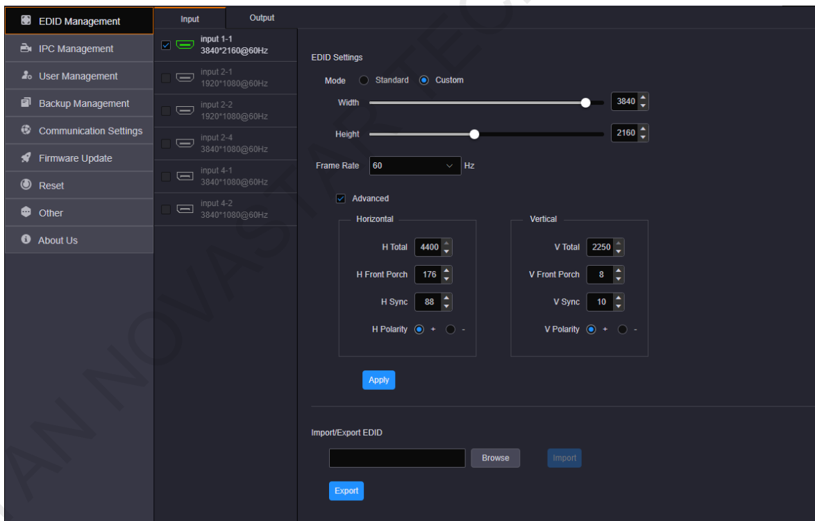
Figure 6-10 Settings
